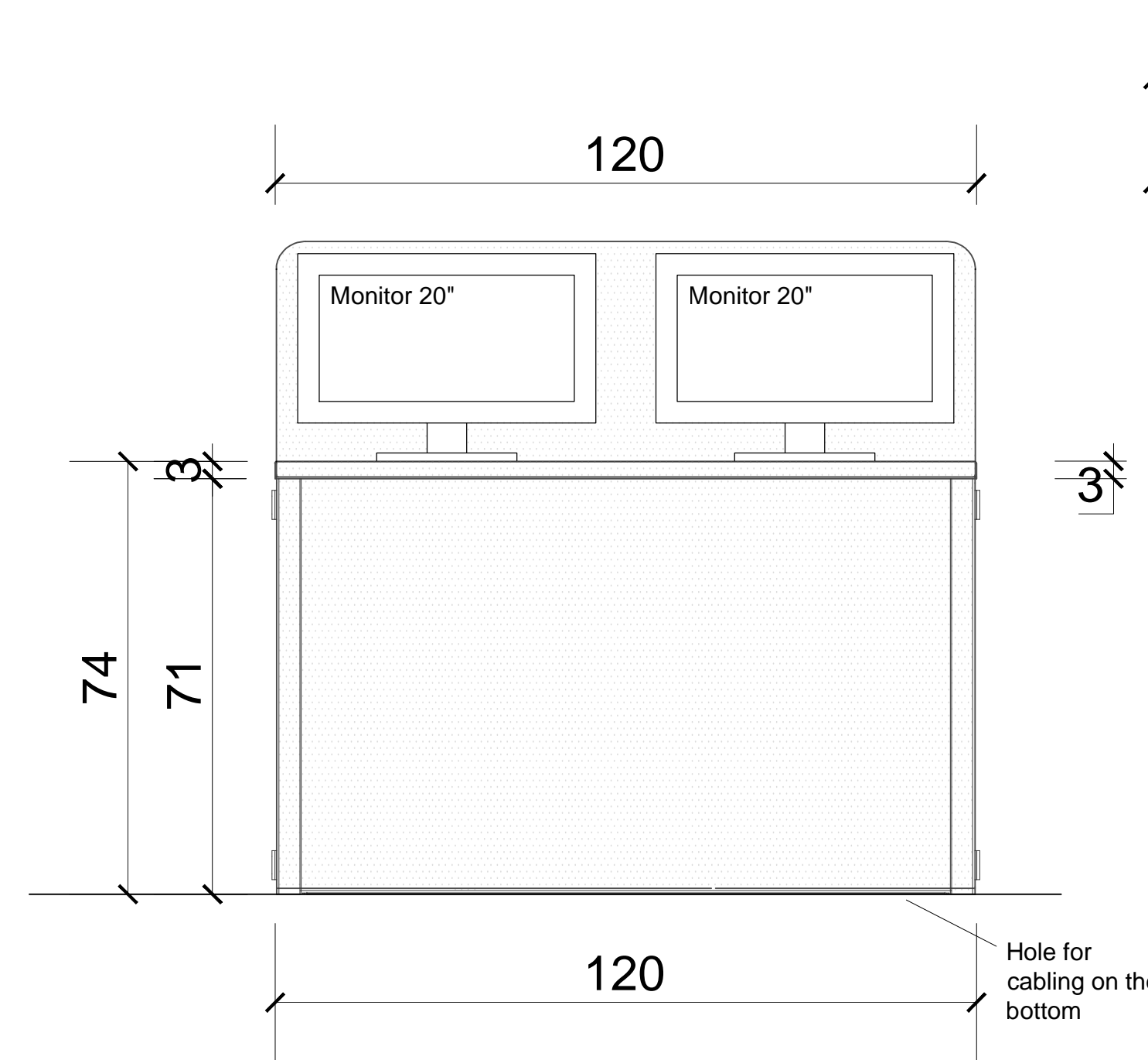
FRONT VIEW
